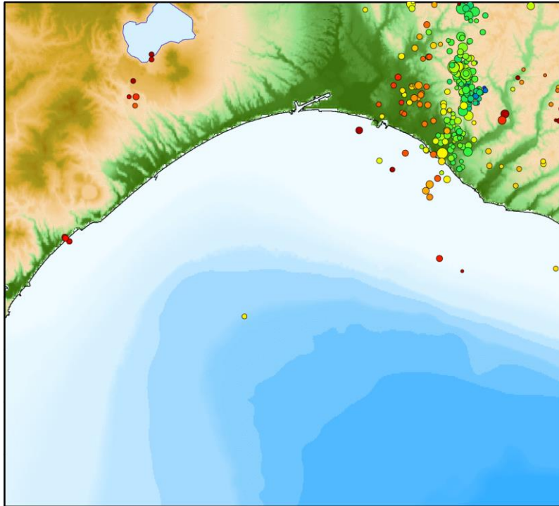
Natural earthquake hypocenter distribution in November 2018
