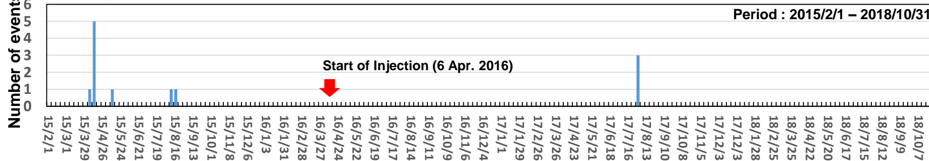
Histogram of detected micro-seismic events
