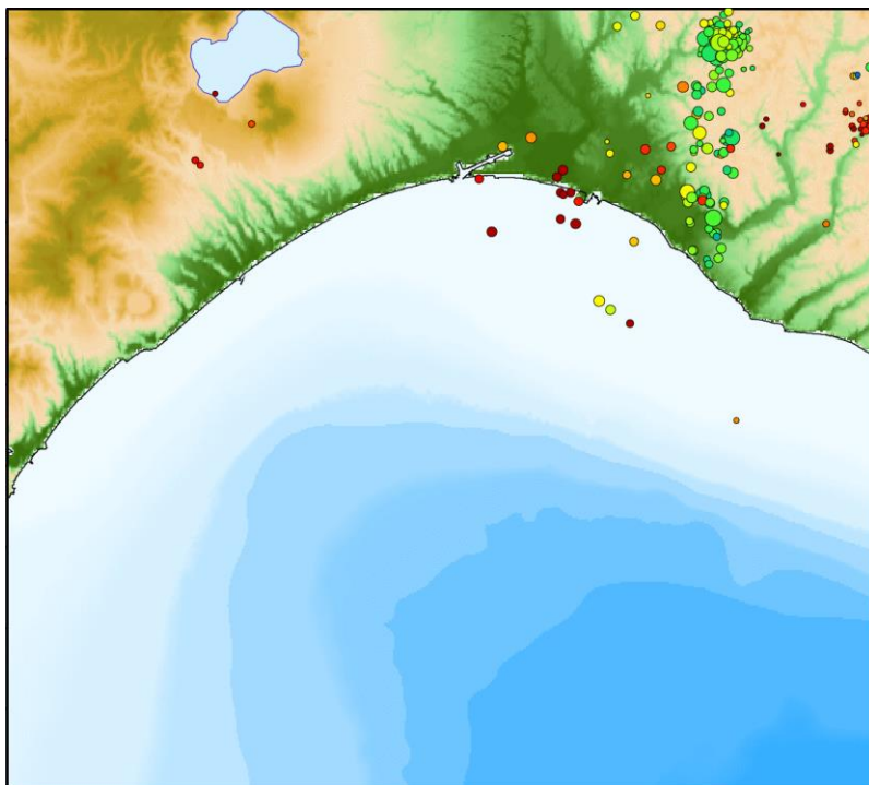
Natural earthquake hypocenter distribution in February 2019
