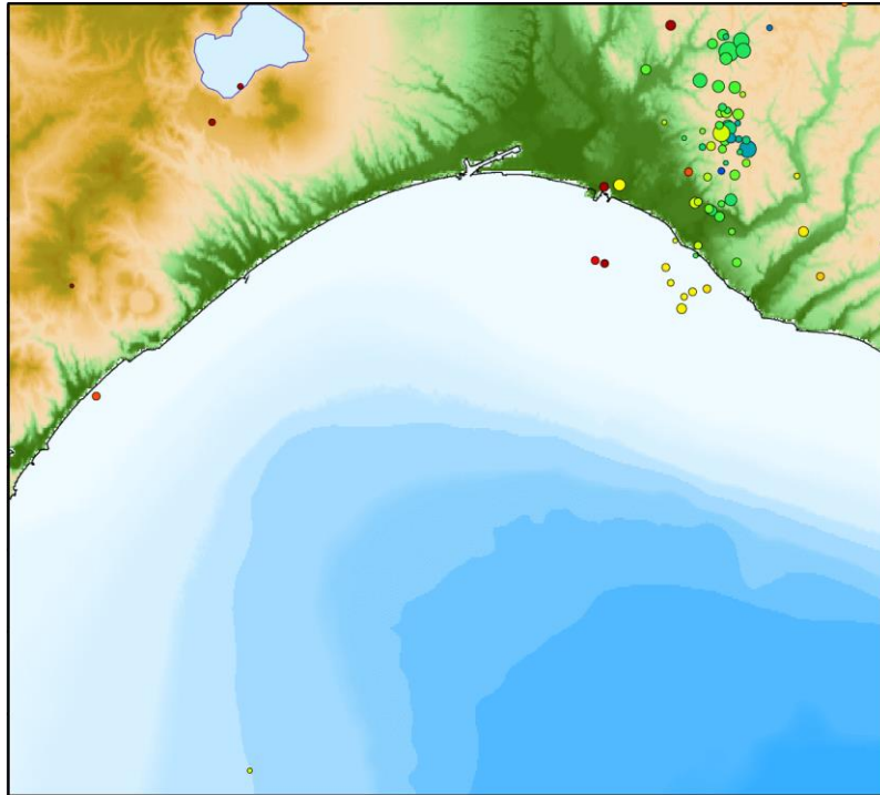
Natural earthquake hypocenter distribution in April 2019
