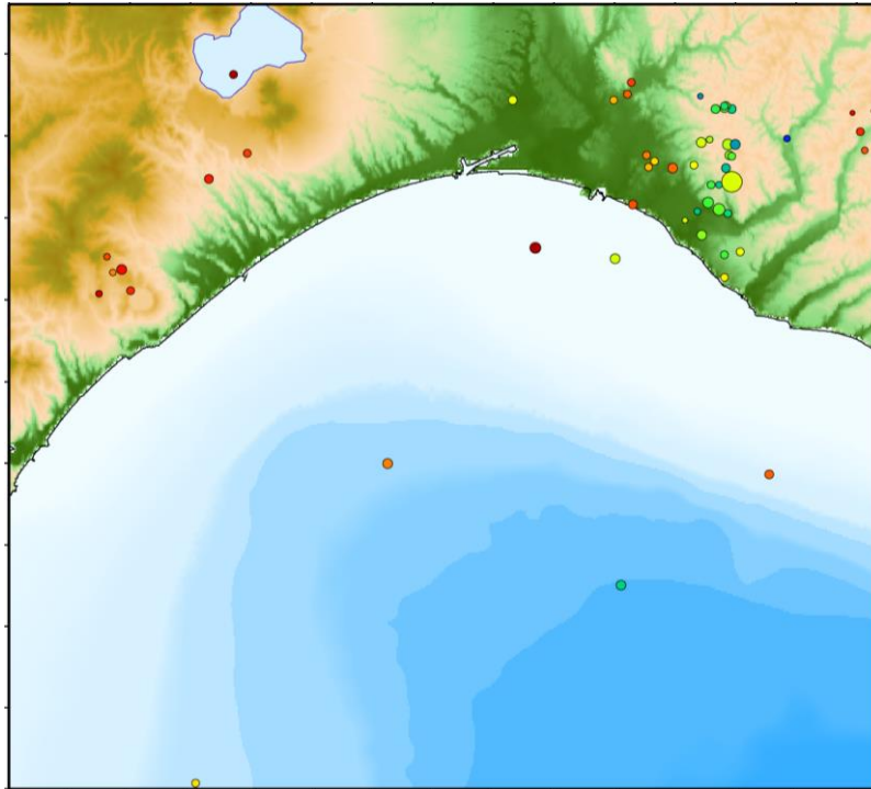
Natural earthquake hypocenter distribution in July 2019
