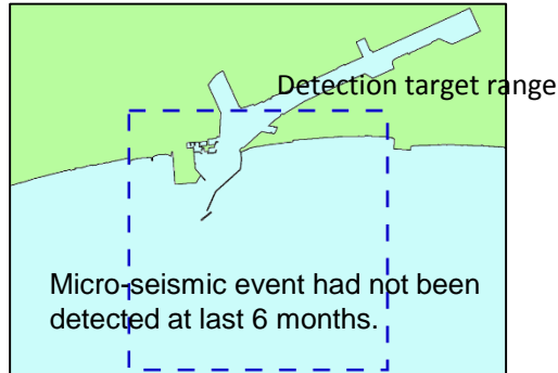
Distribution of the last 6 months (2019/2/1 – 2019/7/31)
