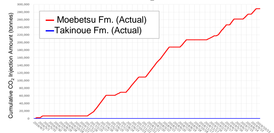
Change of cumulative CO 2 Injection Amount
