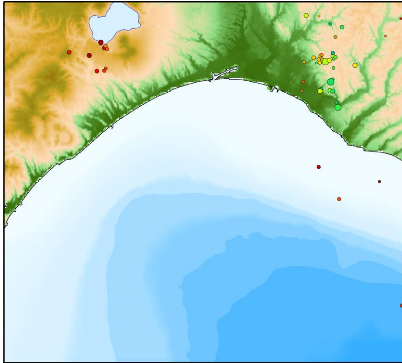
Natural earthquake hypocenter distribution in January 2020
