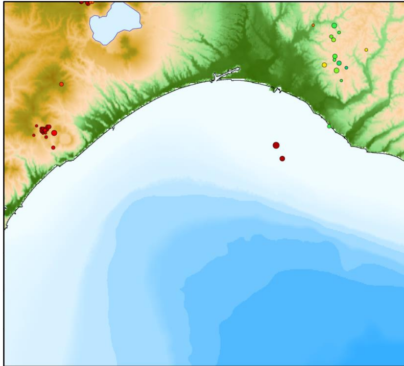
Natural earthquake hypocenter distribution in November 2020
