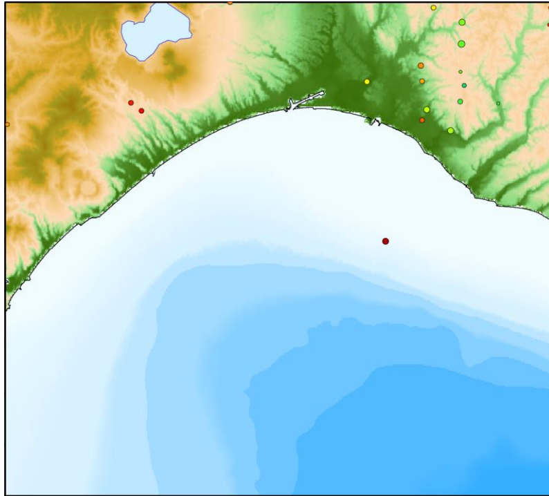
Natural earthquake hypocenter distribution in August 2021
