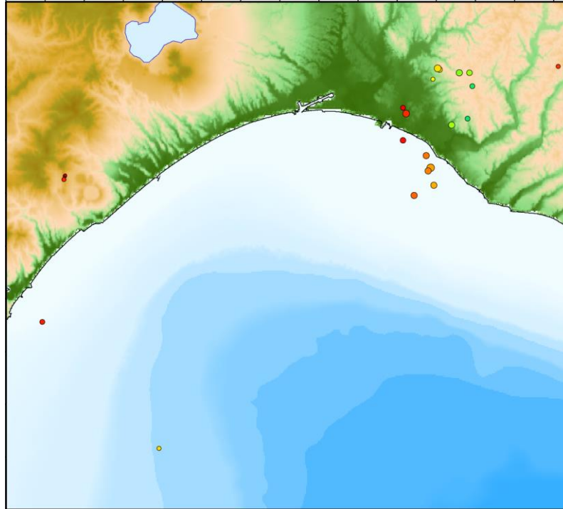
Natural earthquake hypocenter distribution in February 2022
