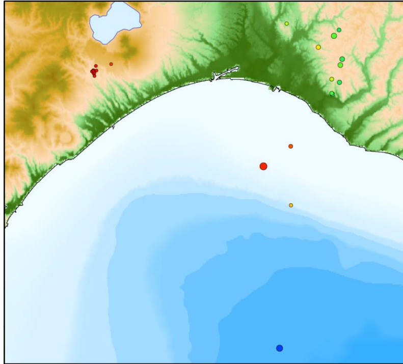
Natural earthquake hypocenter distribution in April 2022
