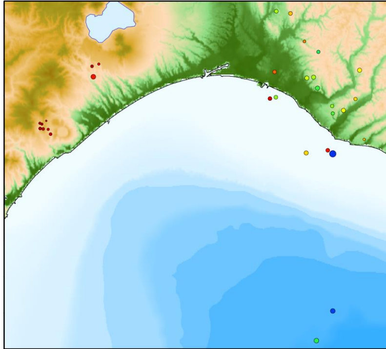
Natural earthquake hypocenter distribution in May 2022
