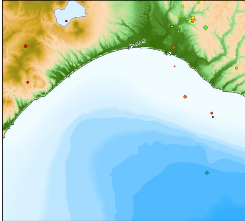
Natural earthquake hypocenter distribution in January 2023
