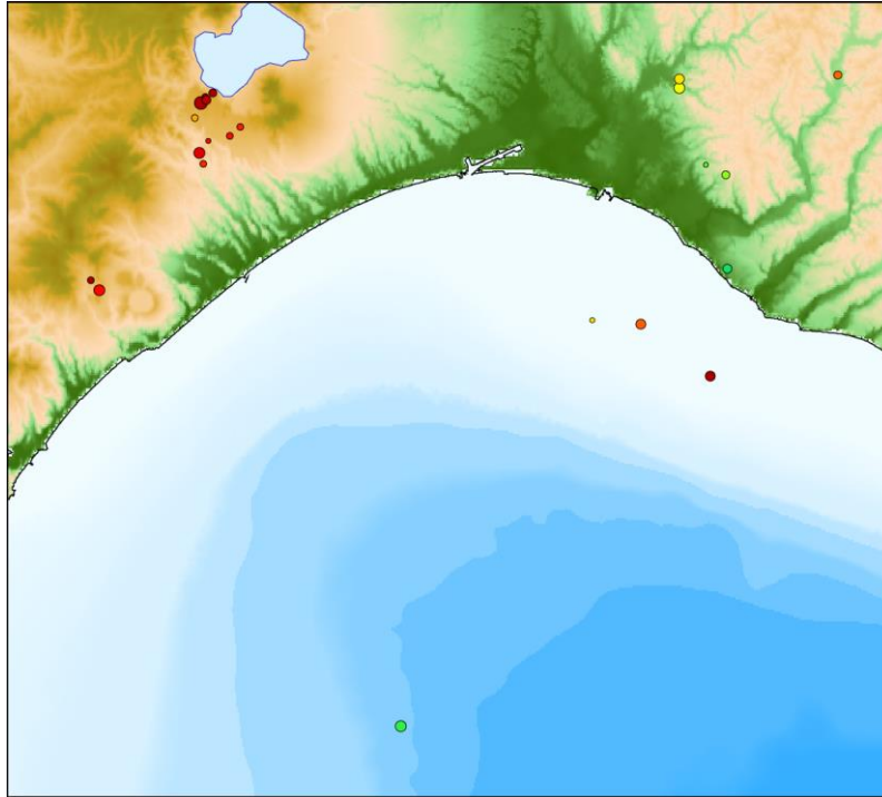
Natural earthquake hypocenter distribution in April 2023
