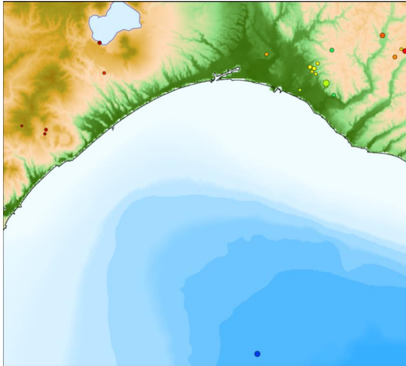
Natural earthquake hypocenter distribution in Jun 2023
