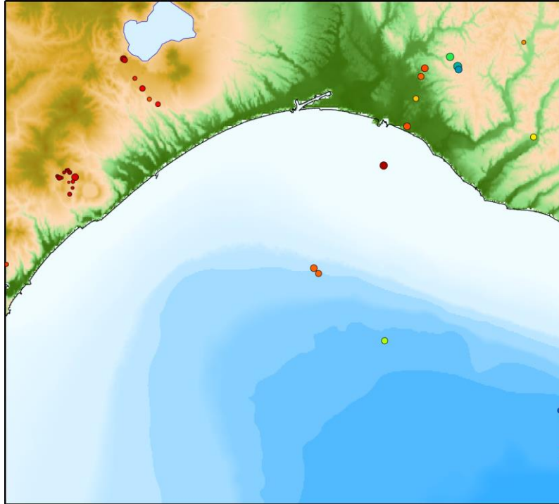
Natural earthquake hypocenter distribution in Dec 2023
