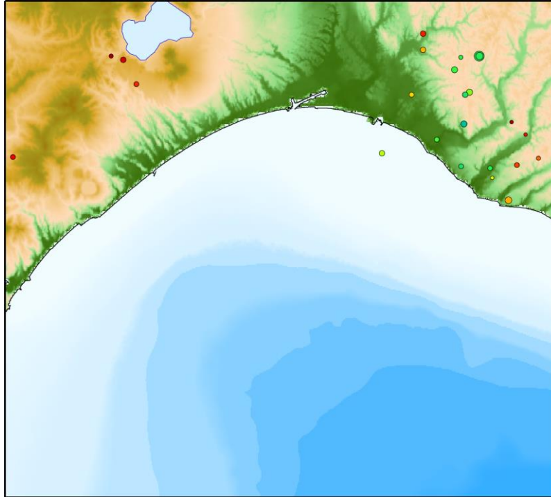
Natural earthquake hypocenter distribution in Mar 2024
