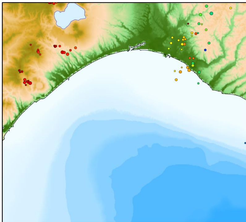
Natural earthquake hypocenter distribution in October 2020
