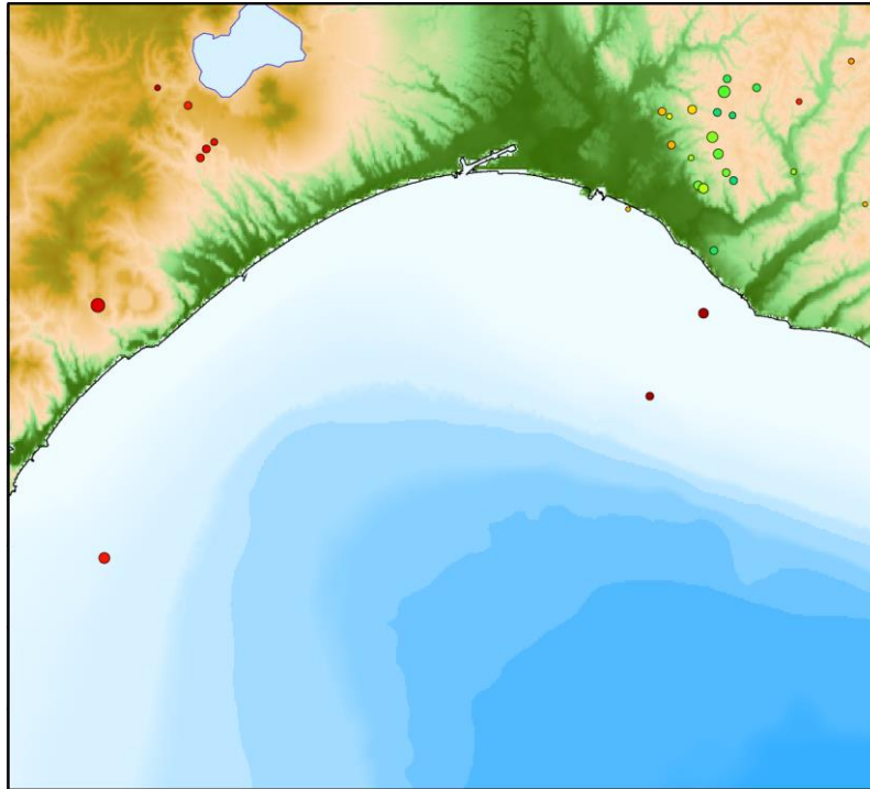
Natural earthquake hypocenter distribution in March 2021
