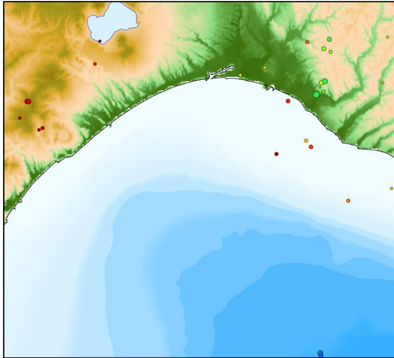
Natural earthquake hypocenter distribution in April 2021
