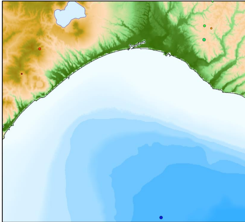
Natural earthquake hypocenter distribution in November 2021
