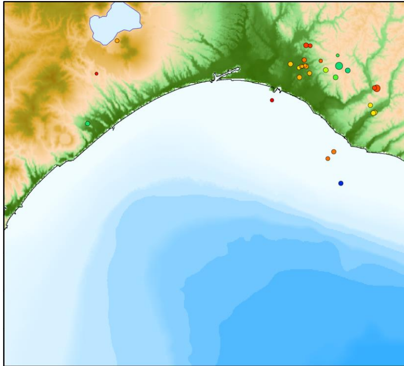
Natural earthquake hypocenter distribution in December 2021
