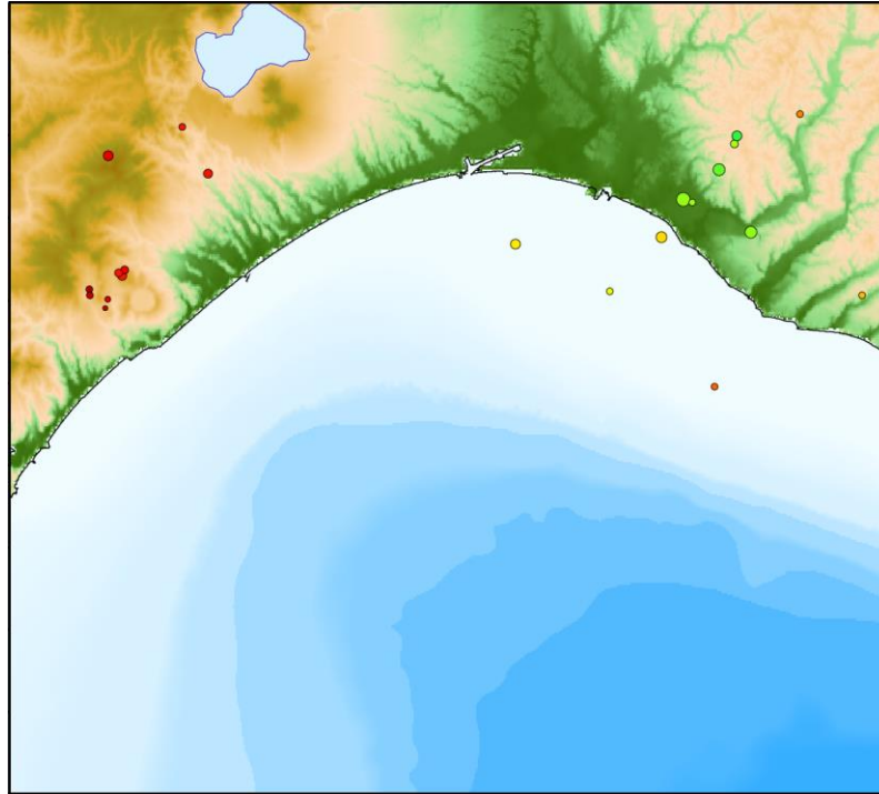
Natural earthquake hypocenter distribution in June 2022
