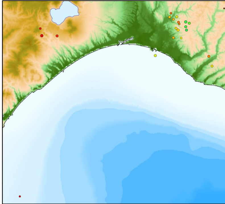
Natural earthquake hypocenter distribution in October 2022
