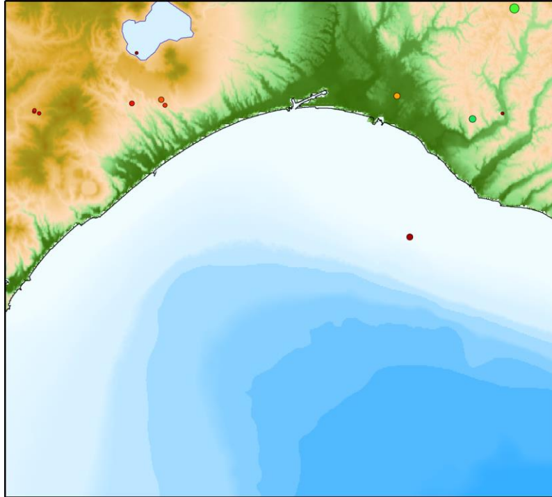
Natural earthquake hypocenter distribution in Dec 2024
