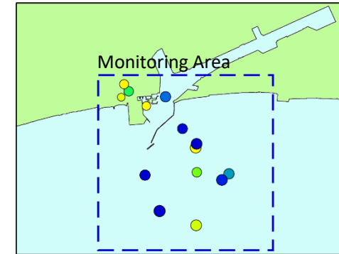
Post-injection events (2019/11/23-2025/8/31)
