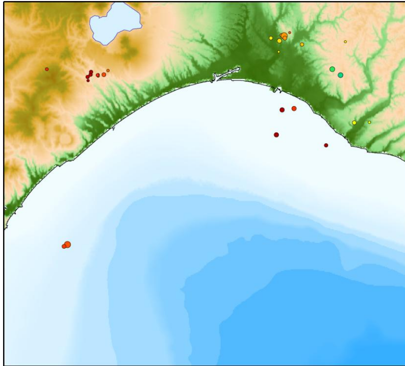
Natural earthquake hypocenter distribution in Aug 2025
