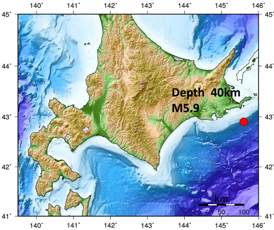
Geomorphic map is prepared from Geographical Survey Institute numerical map 250 m mesh (altitude) and Japan Marine Safety Agency 'Japan Oceanographic Data Center' 500 m mesh water depth data
