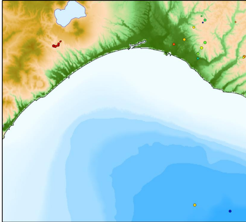
Natural earthquake hypocenter distribution in Sep 2025
