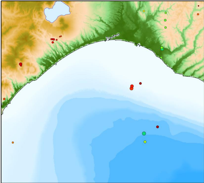
Natural earthquake hypocenter distribution in Oct 2025
