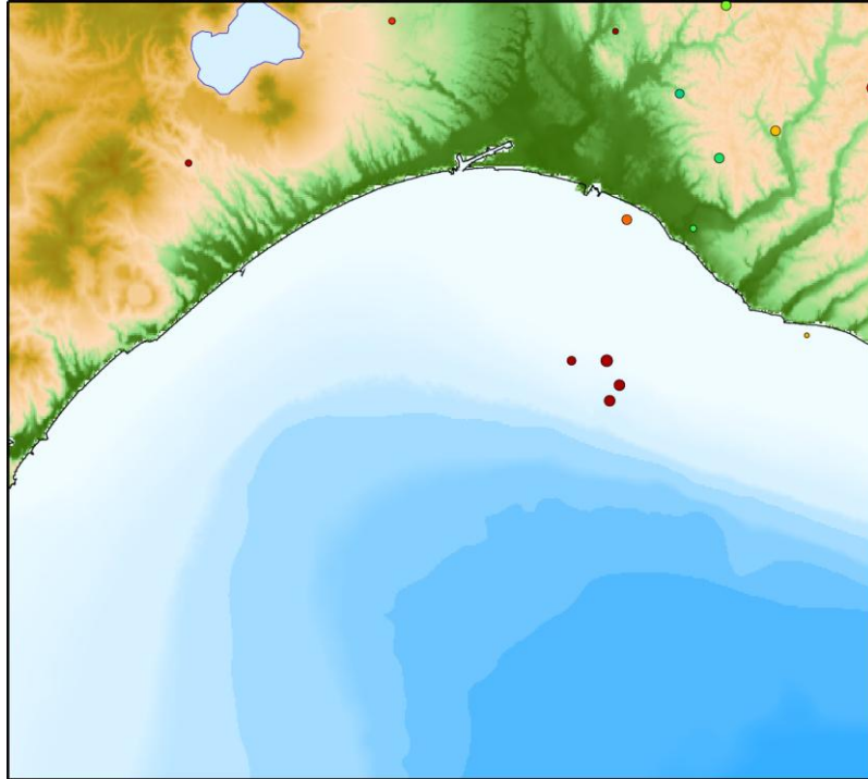
Natural earthquake hypocenter distribution in May 2026
