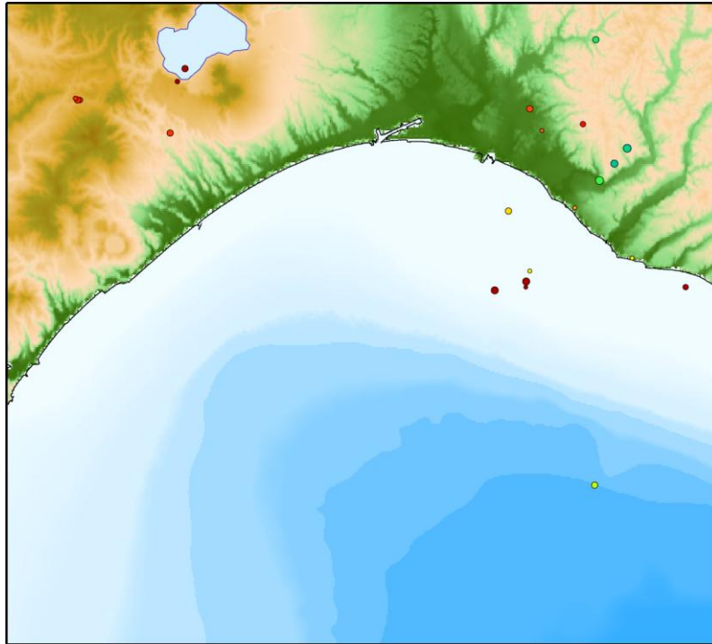
Natural earthquake hypocenter distribution in Jun 2026
