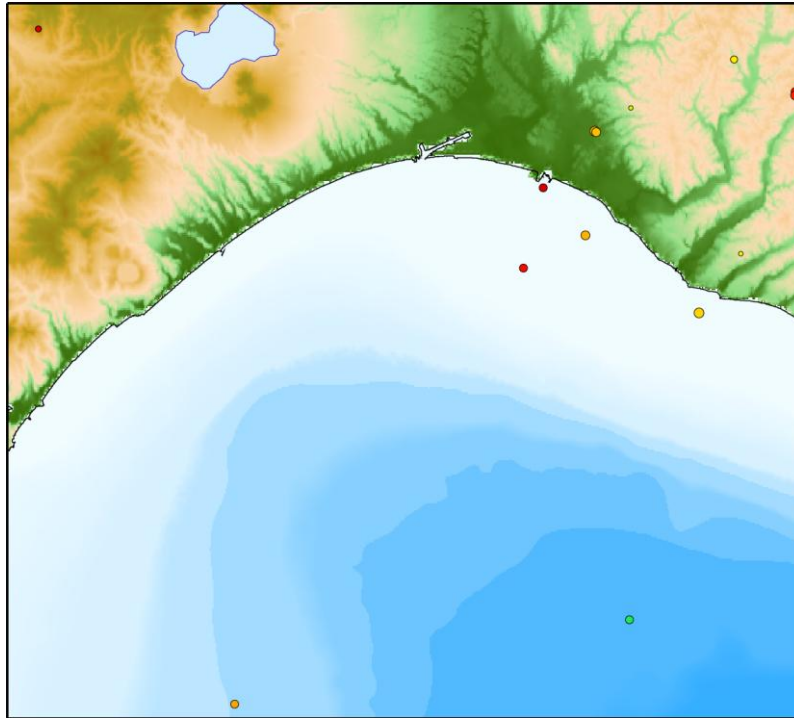
Natural earthquake hypocenter distribution in Aug 2026
